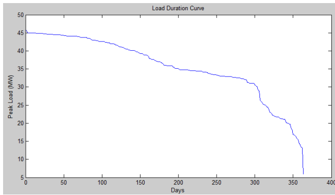
Figure 4. Load duration curve
